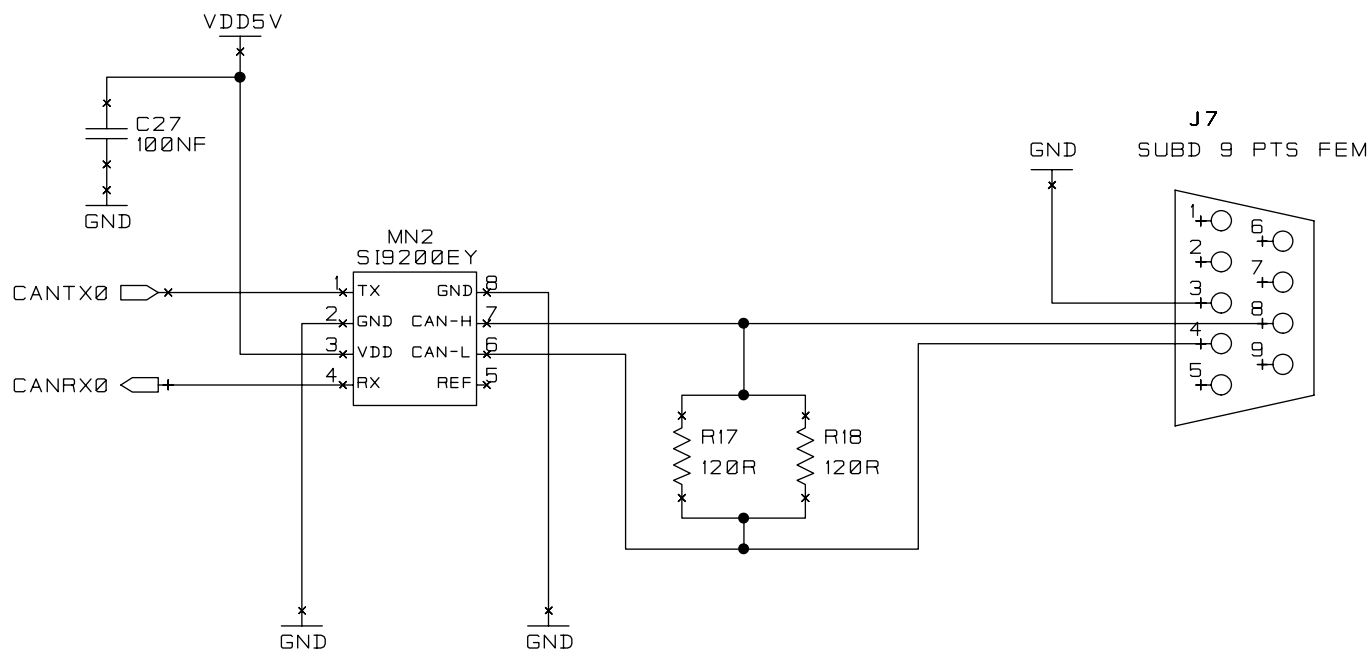
Figure 4-5. CAN Interface
