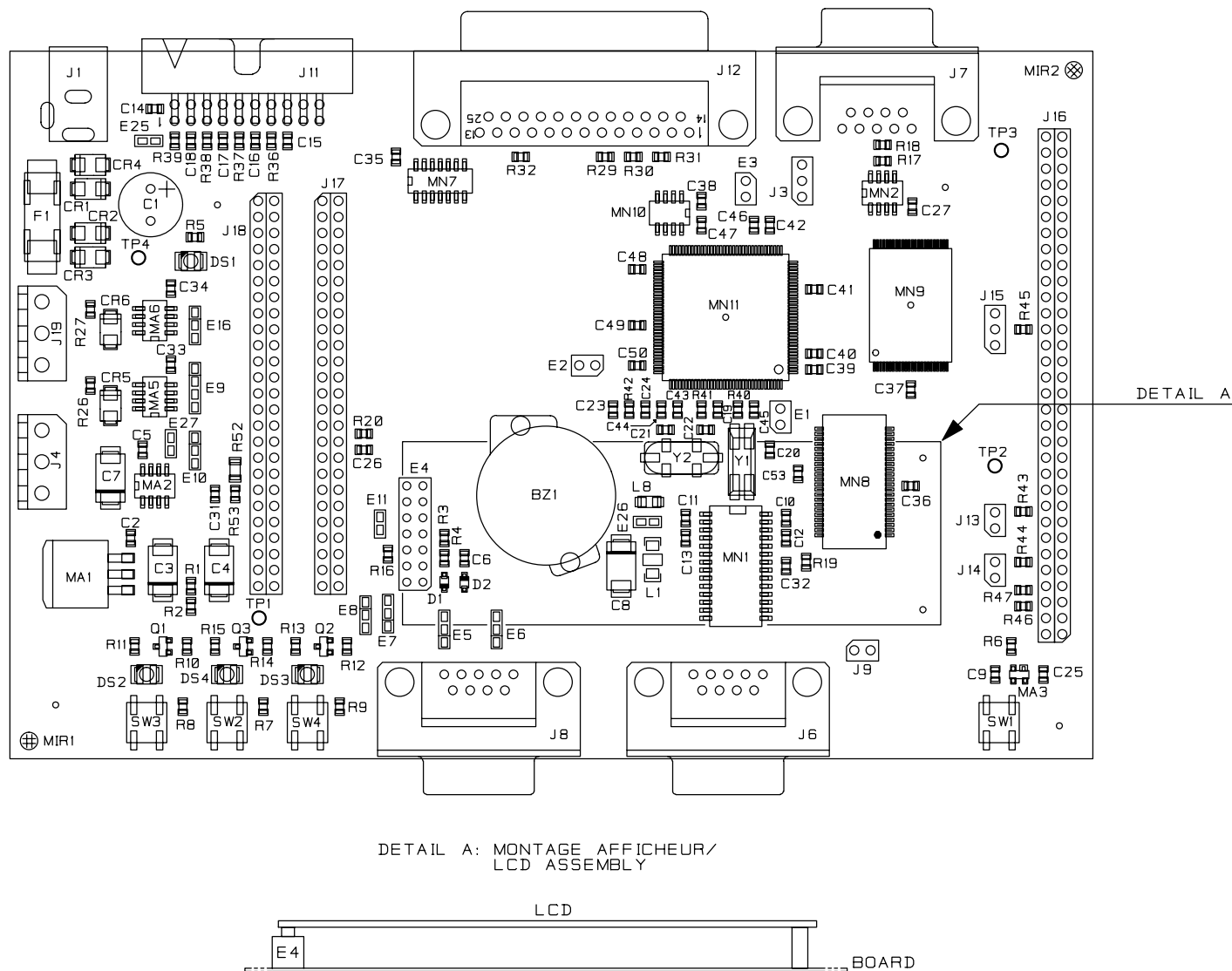
Figure 4-1. Components Side Assembly
