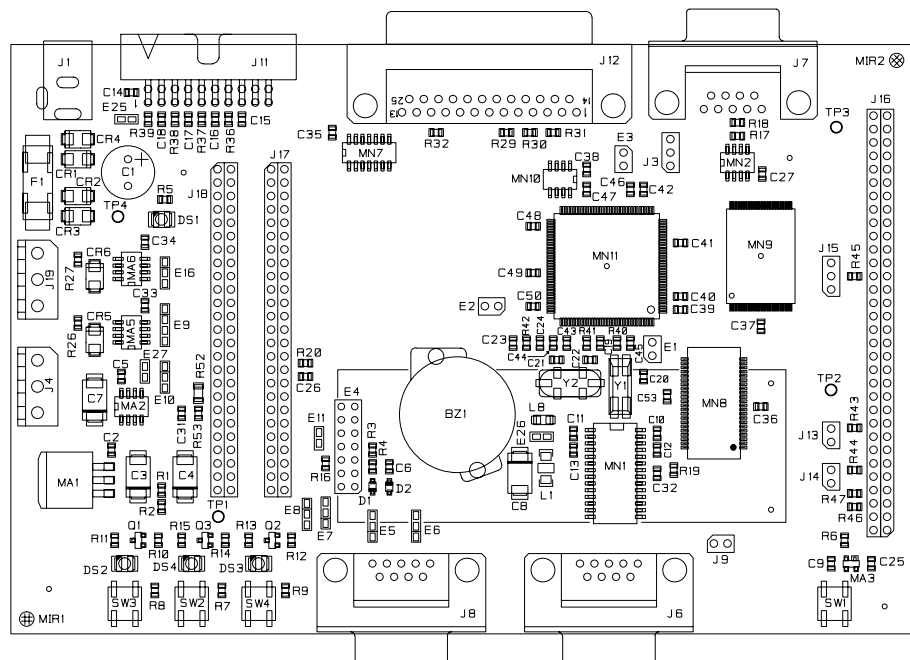
Figure 2-1. Top Level Layout
