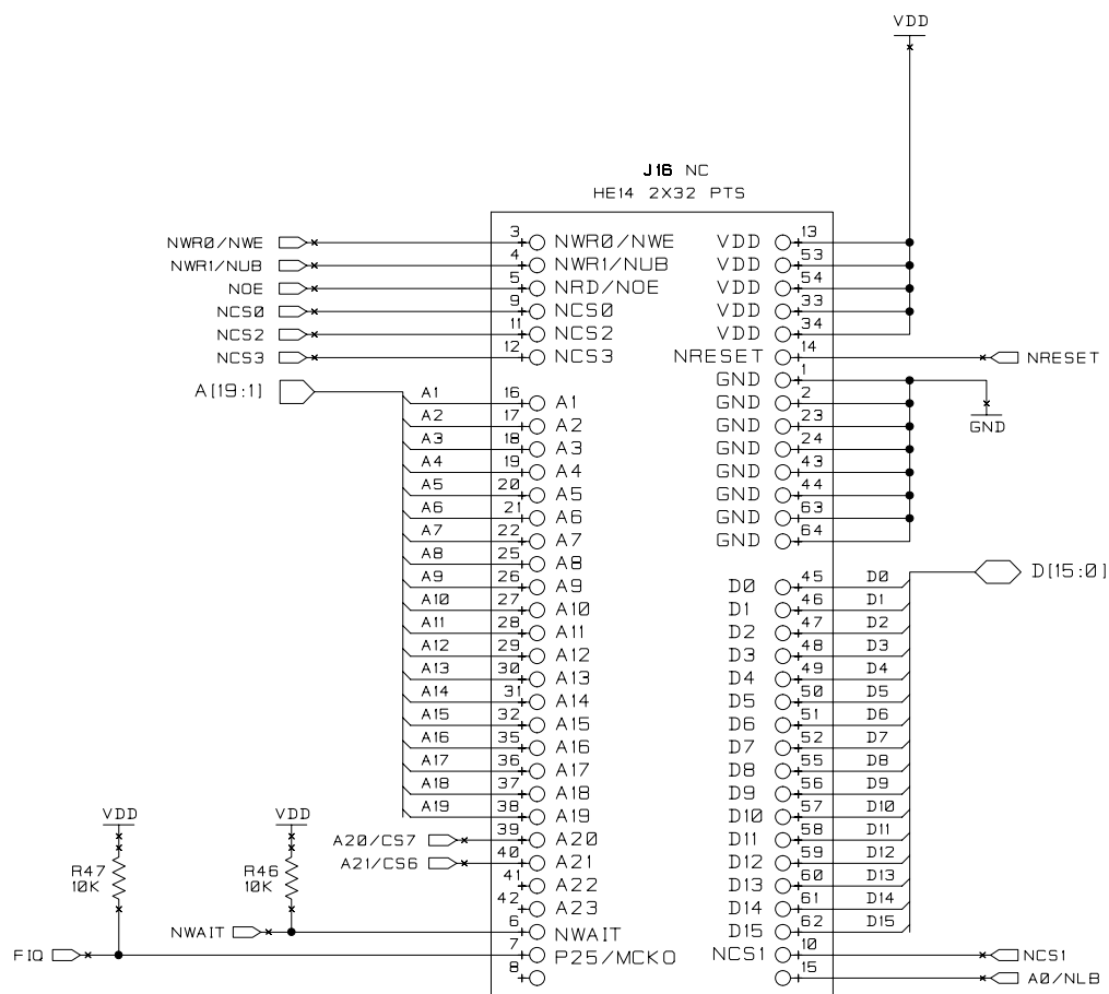
Figure 4-9. EBI Expansion
