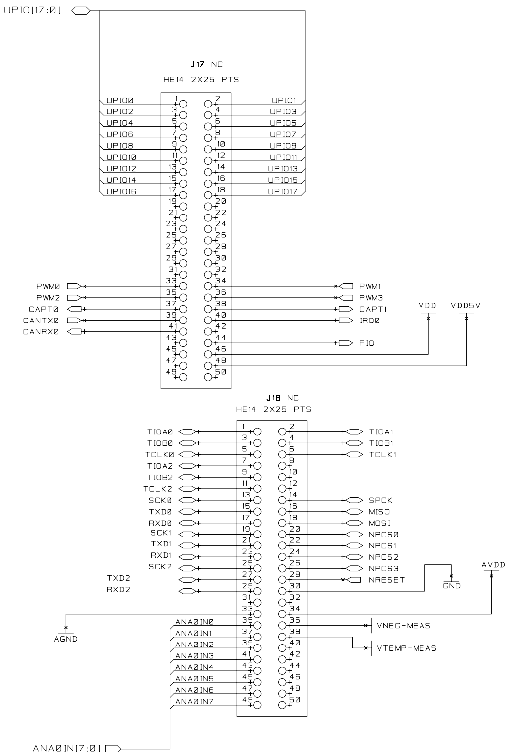
Figure 4-10. Expansion Connector
